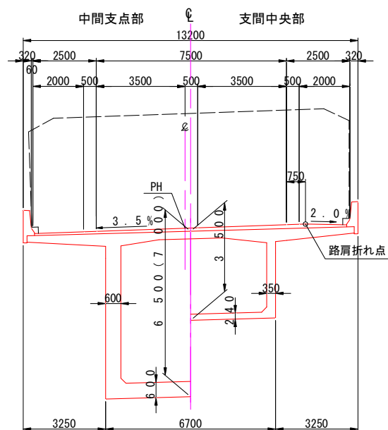
図-1 橋梁断面図
